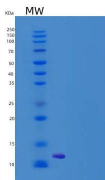
15% SDS PAGE(reduced) analysis of Recombinant Human S100A14 / S114 Protein (His tag)
