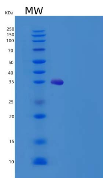
15% SDS PAGE(reduced) analysis of Recombinant Human PHYH Protein
