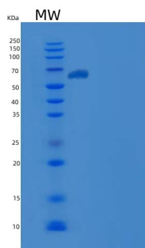
15% SDS PAGE(reduced) analysis of Recombinant Human CDK4 Protein (GST Tag)
