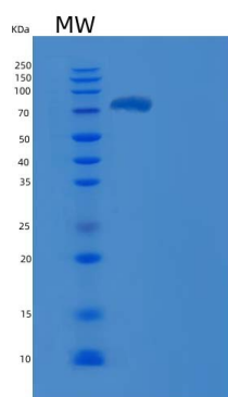
15% SDS PAGE(reduced) analysis of Recombinant Human VRK1 Protein (His & GST tag)
