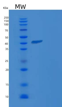
15% SDS PAGE(reduced) analysis of Recombinant Human PRL-2 / PTP4A2 Protein (GST tag)
