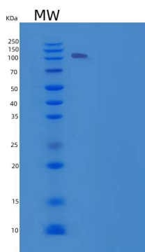
15% SDS PAGE(reduced) analysis of Recombinant Human Semaphorin 5A / SEMA5A Protein (His tag)
