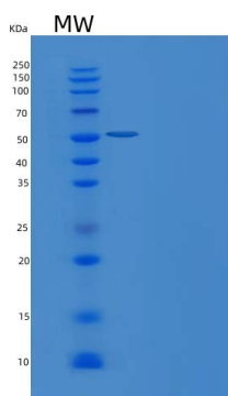
15% SDS PAGE(reduced) analysis of Recombinant Human Chitotriosidase / Chitinase 1 / CHIT1 Protein (His tag)
