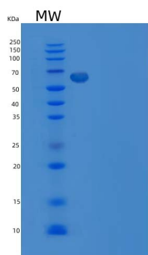
15% SDS PAGE(reduced) analysis of Recombinant Mouse ERK2 / MAPK1 / MAPK2 Protein (His & GST tag)
