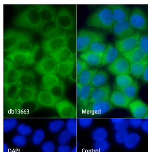
Immunofluorescence analysis of MCF-7 cells labelling MEK1 with db13663.
