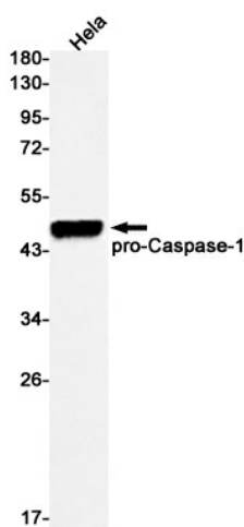
Western blot detection of Caspase-1 in HeLa cell lysates using Caspase-1 antibody(1:500 diluted).
